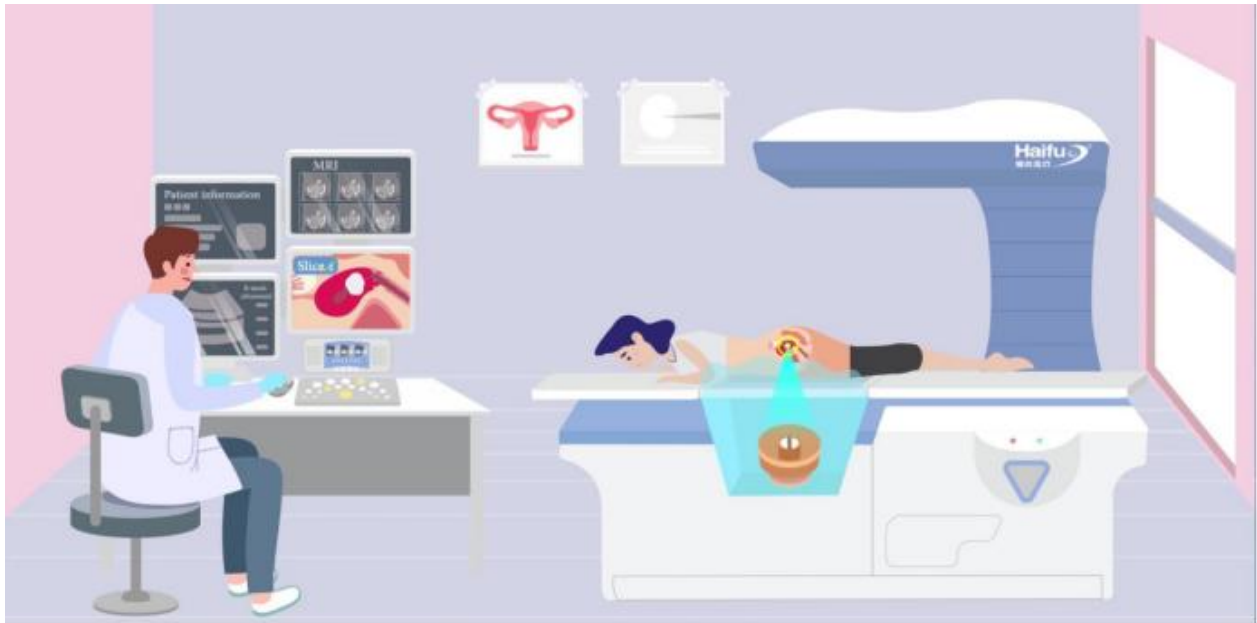
Treatment Scenario (Model JC200)
